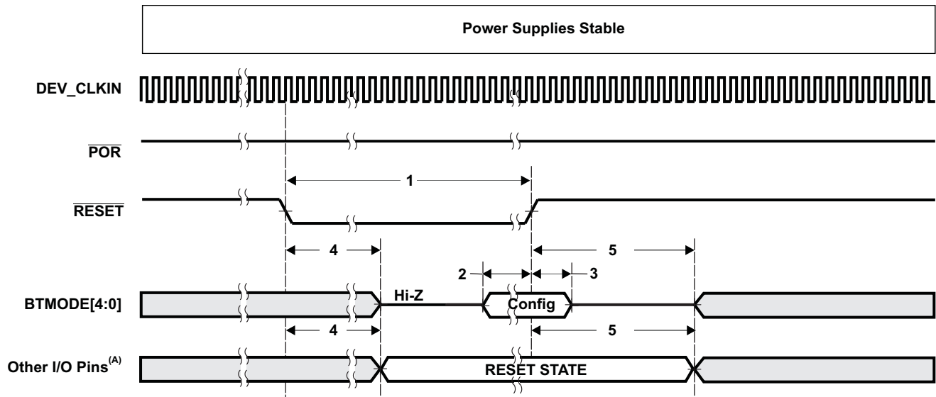
Figure 7-2. Power-Up Timing
